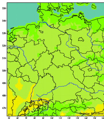
REMO
